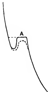
FIG. 74.—Effect of undercooling on cooling curve.
